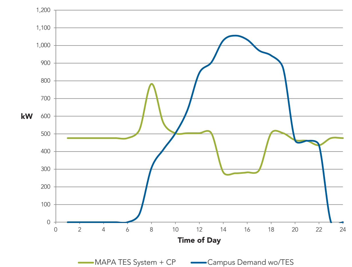
OPTION 2—CAMPUS ELECTRICAL DEMAND
