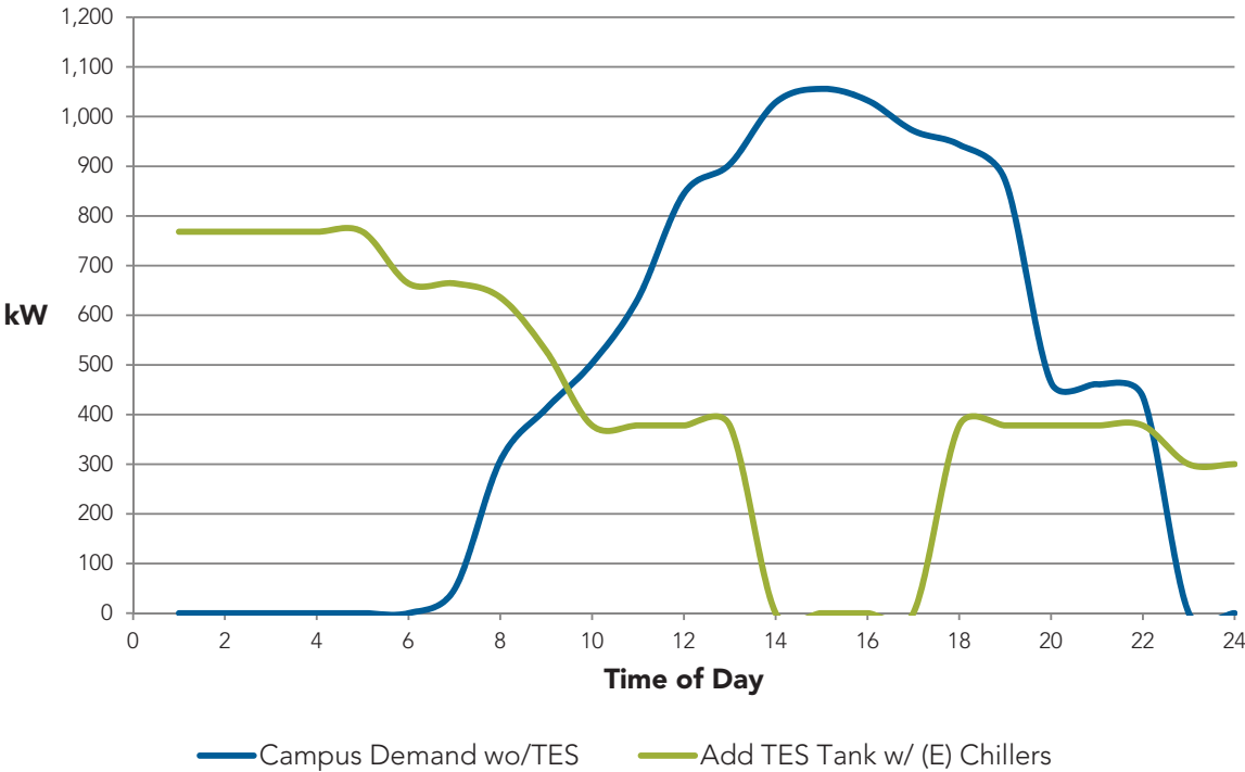
OPTION 4—CAMPUS ELECTRICAL DEMAND
