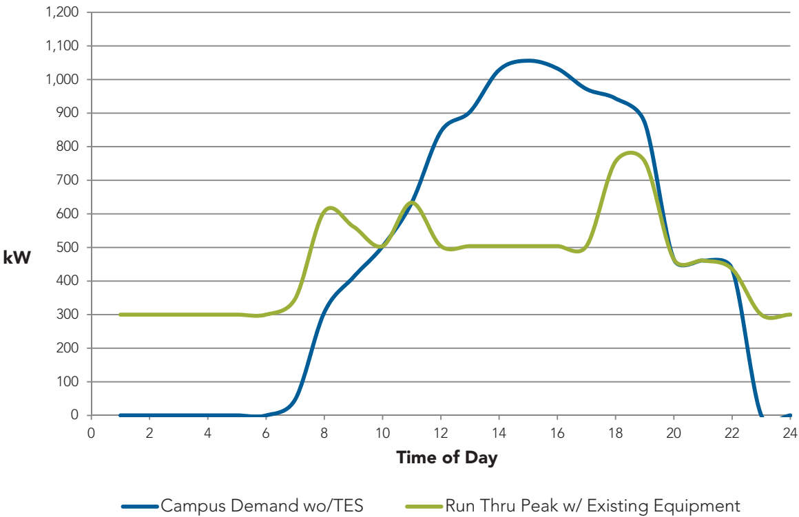
OPTION 1—CAMPUS ELECTRICAL DEMAND
